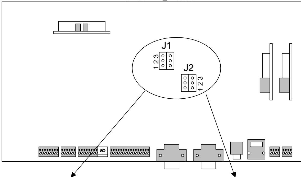
Jumpers on Motherboard for EXTERNAL
