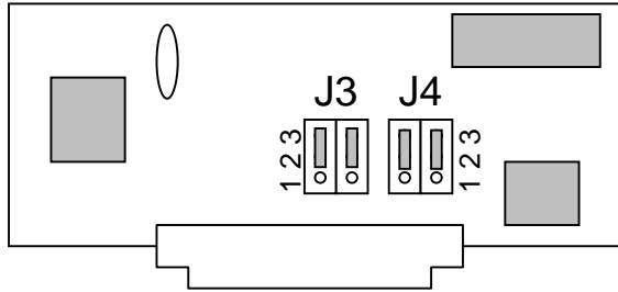
Jumpers on MSo for EXTERNAL
