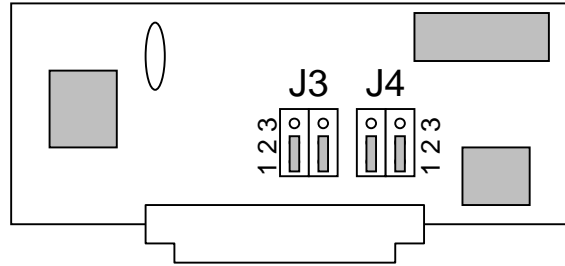
Jumpers on MSo for INTERNAL
